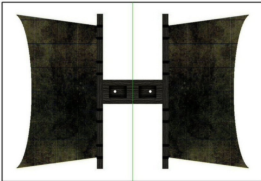
MAIN TOP GALLANT SAIL \
