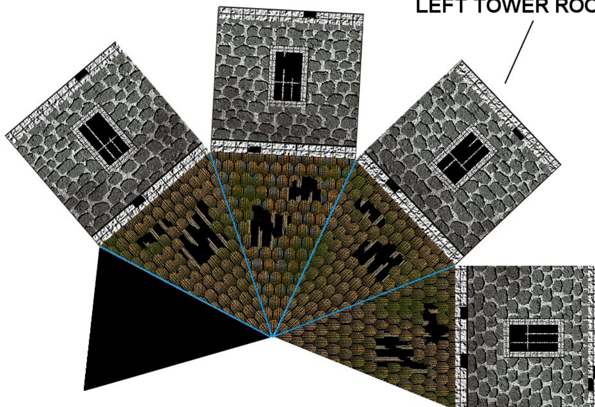
LEFT TOWER ROOF
